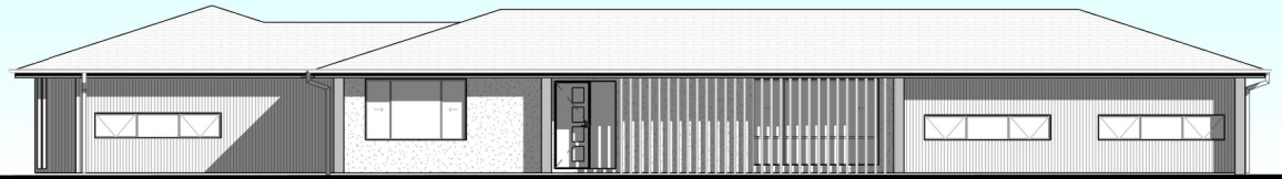
PROPOSED SOUTH ELEVATION
